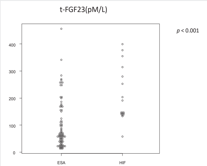
Figure 1: Serum t-FGF23 levels. t-FGF23: total Fibroblast Growth Factor-23; Erythropoiesis-Stimulating Agent; HIF: Hypoxia-Inducible Factor
